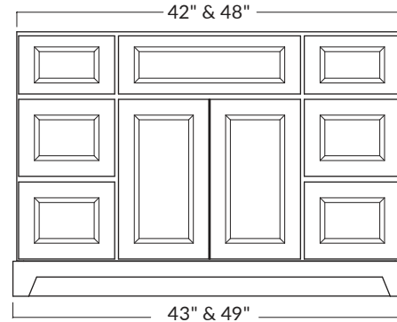
42" OR 48" SINGLE SINK
