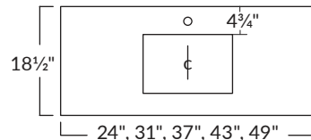
SINK POSITIONING WITH STONE TOPS (NOTE: The stone top opening is 15 1/8" x 10")
