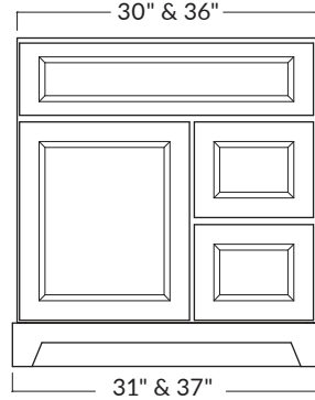
30" OR 36" RIGHT DRAWER SINGLE SINK
